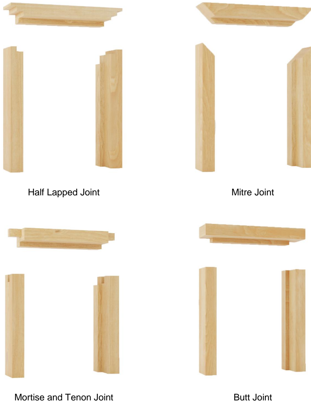
Figure 7.4 – Frame jointing detail
