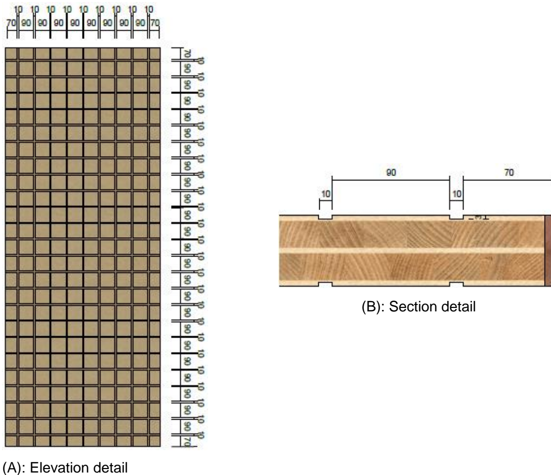
Figure 5.4 – Decorative groove detail on Leaf 1
