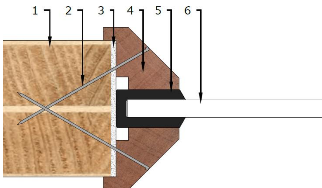
Figure 6.9 – Lorient System-63Ø – for circular glazing installation detail
