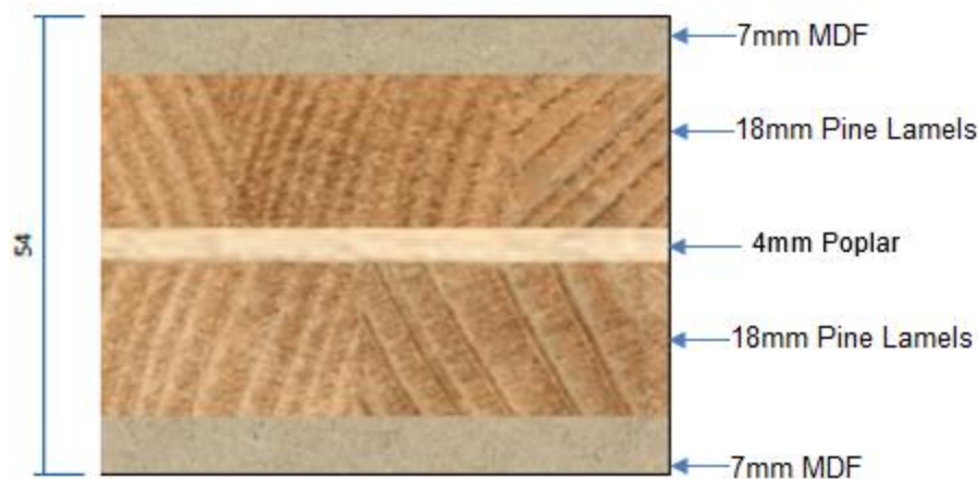
Figure 5.3 – Leaf 2 – Stredor 54 with MDF facing
