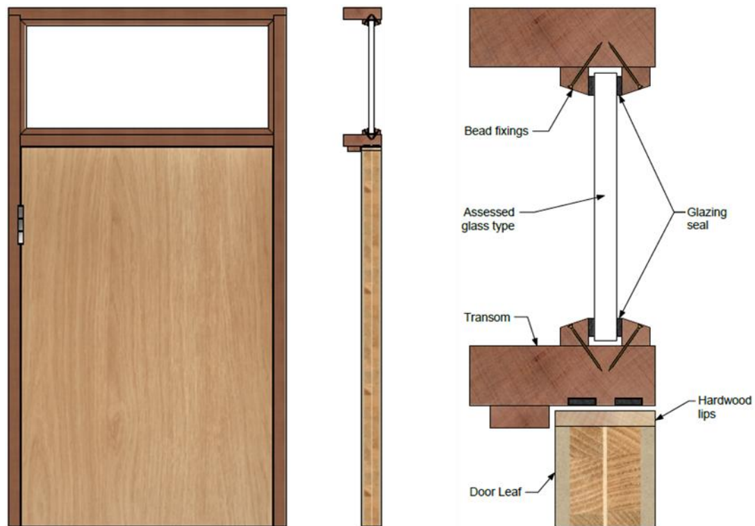
Figure 8.2 – Fanlight detail
