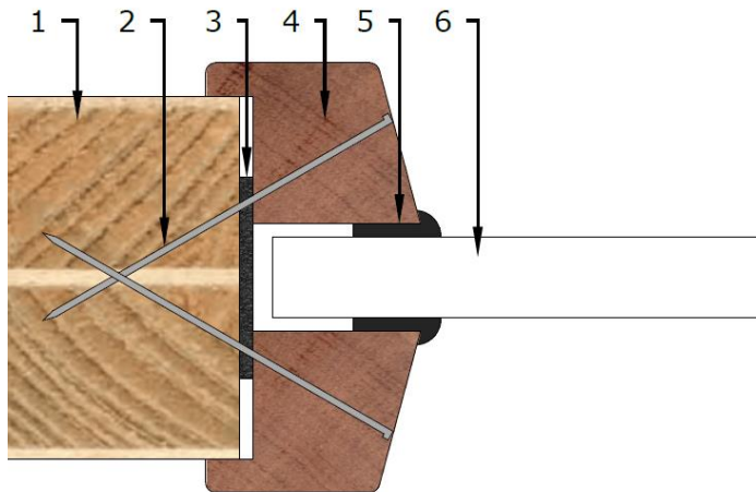
Figure 6.13 – STS104SG/ST302GL installation detail
