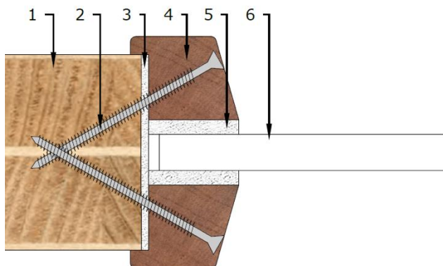
Figure 6.11 – ISL 60 Plus installation detail
