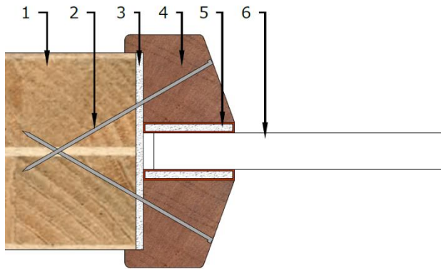
Figure 6.8 – Mann McGowan Pyroglaze 60 installation detail
