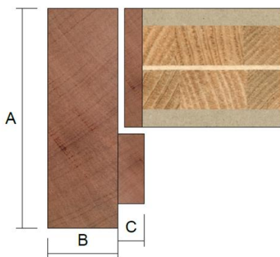
Figure 7.1 – Standard frame detail
