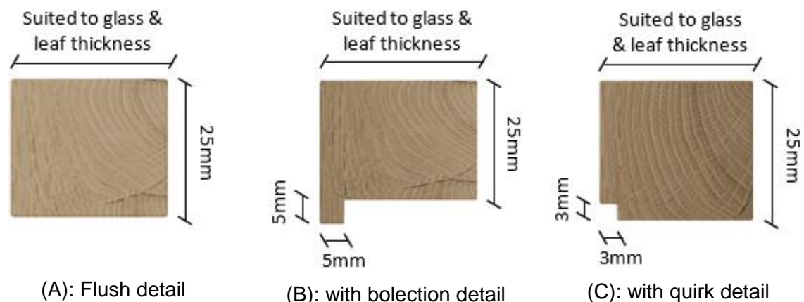
Figure 6.1 – Square bead detail
