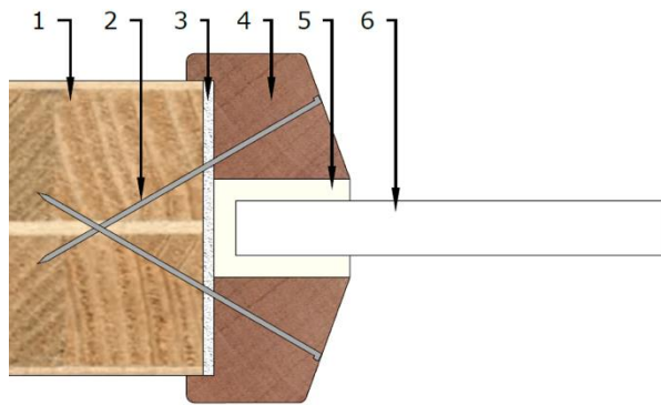
Figure 6.5 – Sealmaster Fireglaze Mastic installation detail
