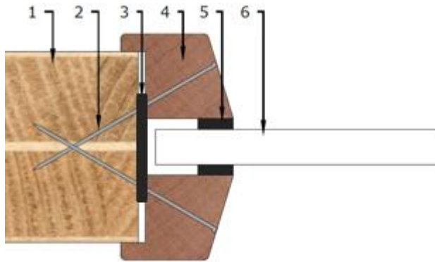
Figure 6.10 – Sealed Tight Solutions STS105GT3 / STS302 installation detail
