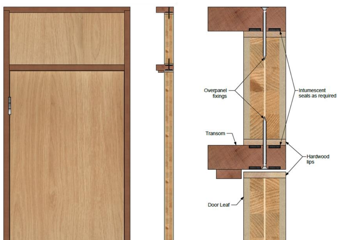
Figure 8.1 – Transomed overpanel detail
