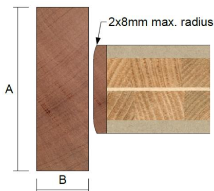
Figure 7.3 – Square frame detail
