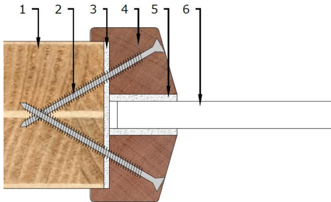
Figure 6.12 – Sealmaster Fireglaze installation detail
