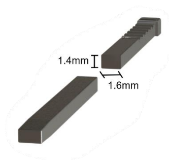
Figure 6.3 – Rectangular pin detail – minimum dimension 1.4mm
