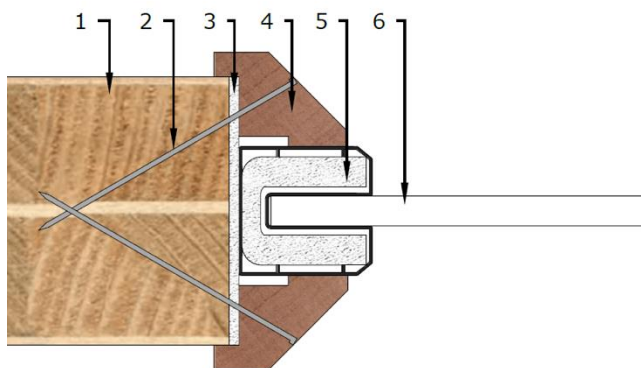
Figure 6.7 – Lorient System-90 Plus installation detail
