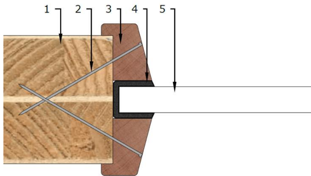
Figure 6.6 – Lorient System-36 Plus installation detail
