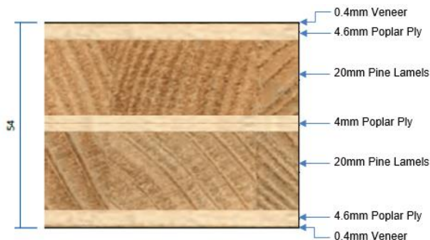
Figure 5.2 – Leaf 1 (Type 2) Stredor 54 with plywood facing
