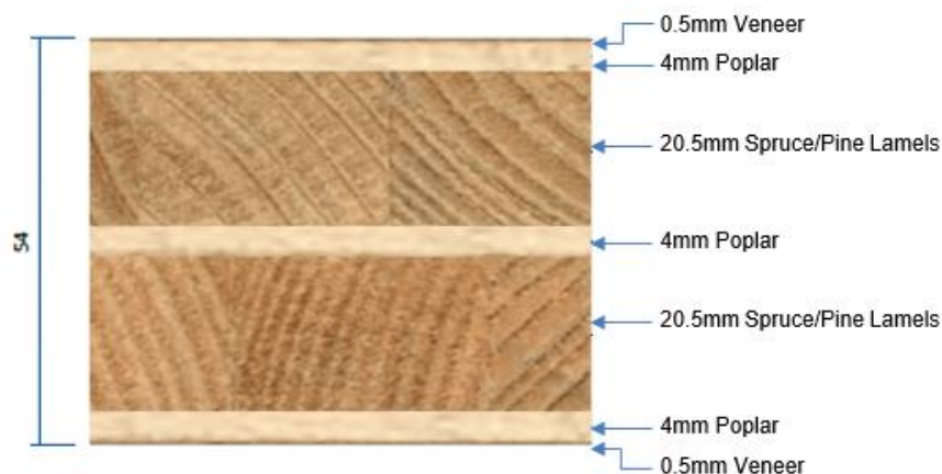
Figure 5.1 – Leaf 1 (Type 1) Stredor 54 with plywood facing
