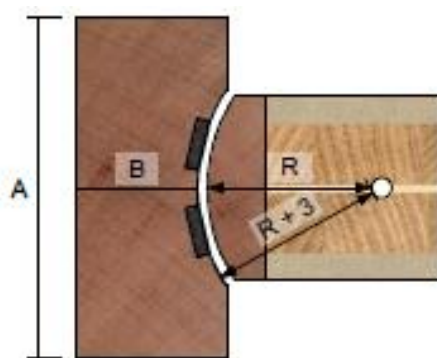
Figure 7.2 – Scalloped frame detail
