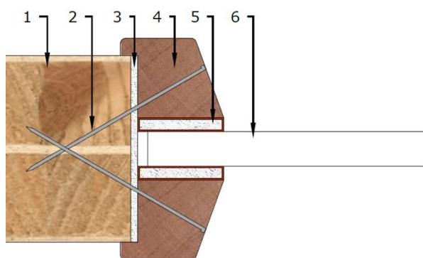
Figure 6.4 – ISL Therm-A-Glaze 60 installation detail
